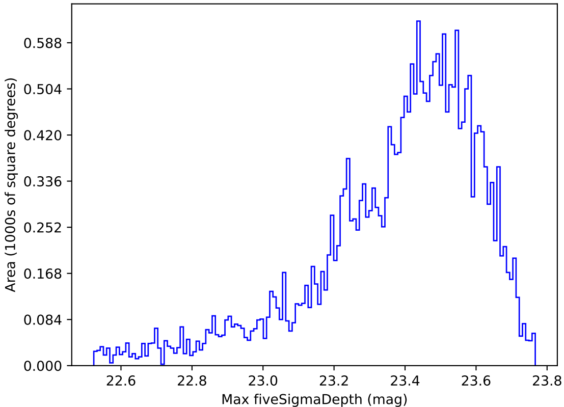
noroll_mjdp365_v3.4_10yrs Yr 1 z band: Max fiveSigmaDepth
