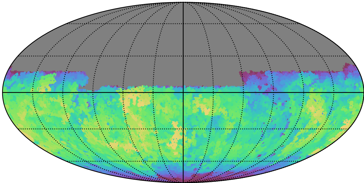
noroll_mjdp365_v3.4_10yrs Yr 1 y band: Max fiveSigmaDepth
