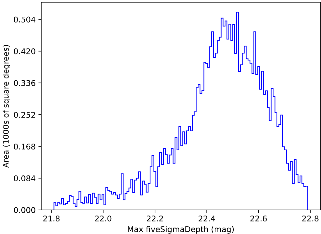
noroll_mjdp365_v3.4_10yrs Yr 1 y band: Max fiveSigmaDepth
