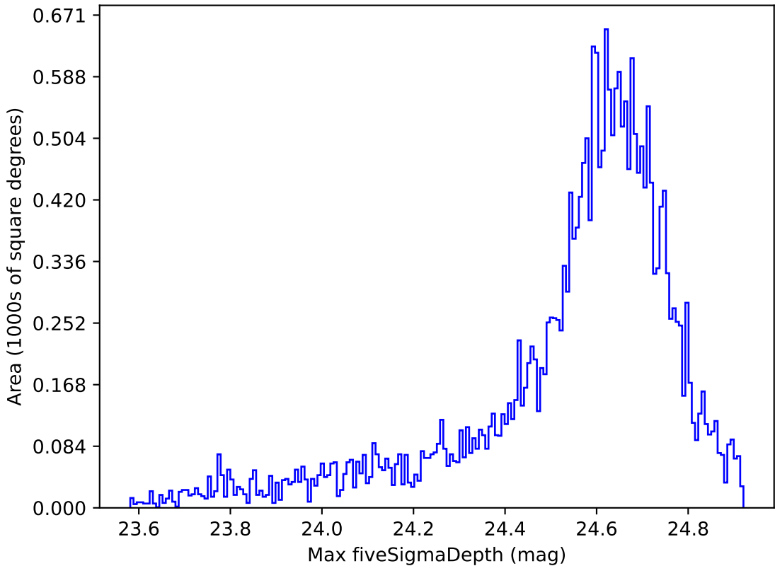
noroll_mjdp365_v3.4_10yrs Yr 1 r band: Max fiveSigmaDepth
