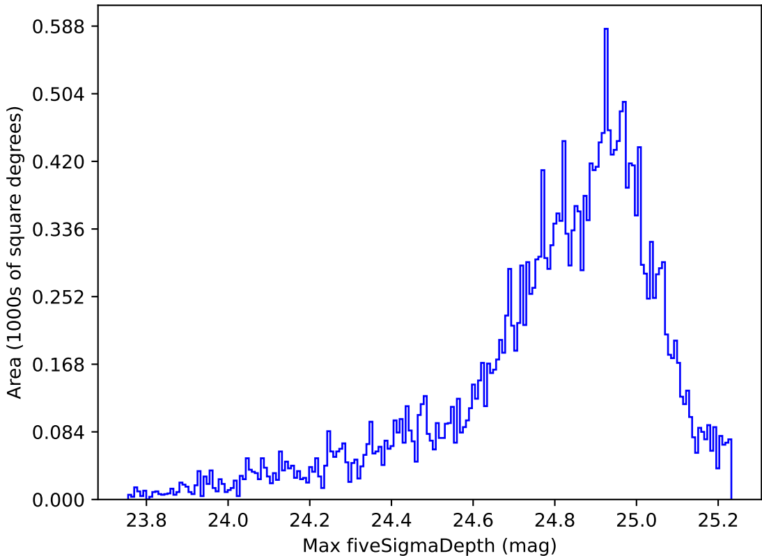
noroll_mjdp365_v3.4_10yrs Yr 1 all bands: Max fiveSigmaDepth
