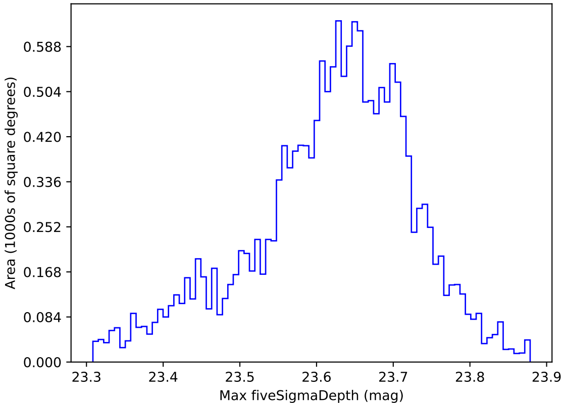
noroll_mjdp365_v3.4_10yrs WFD z band: Max fiveSigmaDepth
