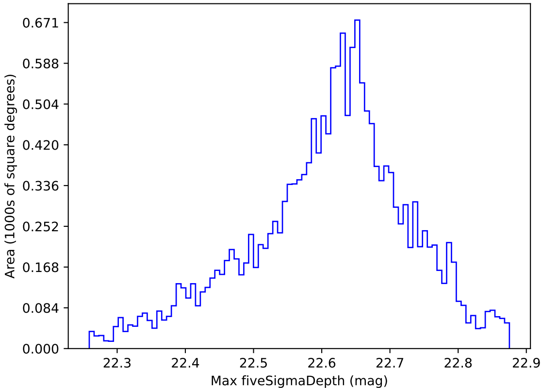
noroll_mjdp365_v3.4_10yrs WFD y band: Max fiveSigmaDepth
