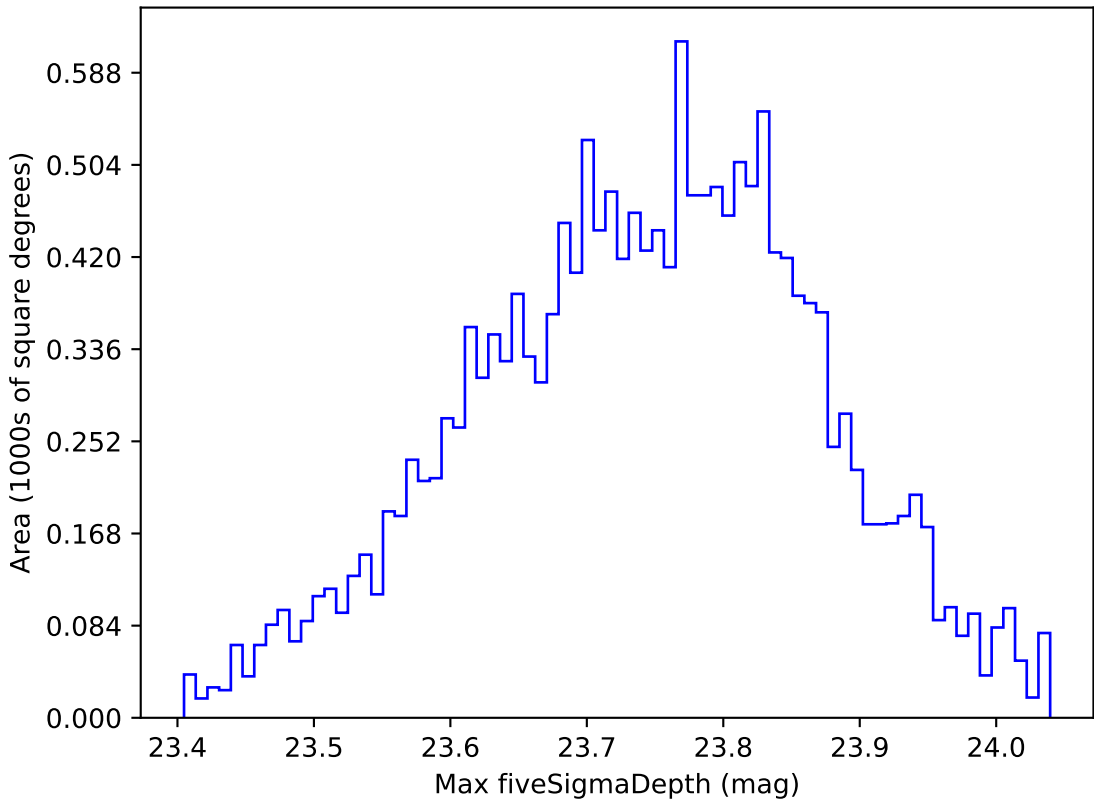
noroll_mjdp365_v3.4_10yrs WFD u band: Max fiveSigmaDepth
