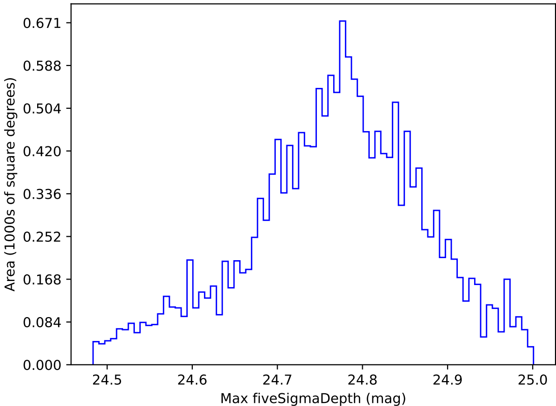
noroll_mjdp365_v3.4_10yrs WFD r band: Max fiveSigmaDepth
