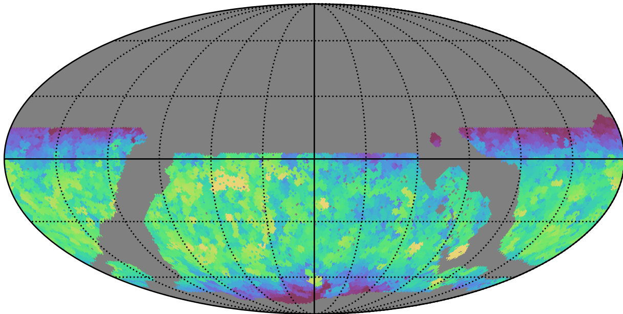
noroll_mjdp365_v3.4_10yrs WFD i band: Max fiveSigmaDepth
