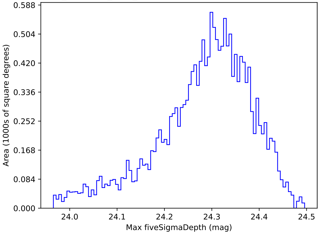
noroll_mjdp365_v3.4_10yrs WFD i band: Max fiveSigmaDepth
