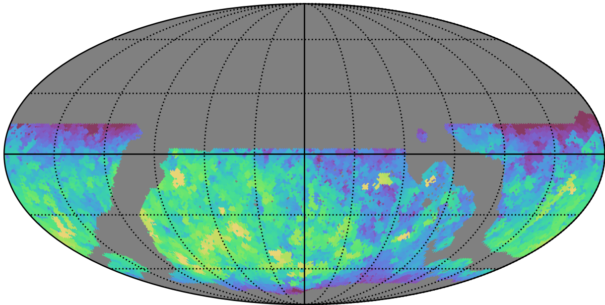
noroll_mjdp365_v3.4_10yrs WFD g band: Max fiveSigmaDepth
