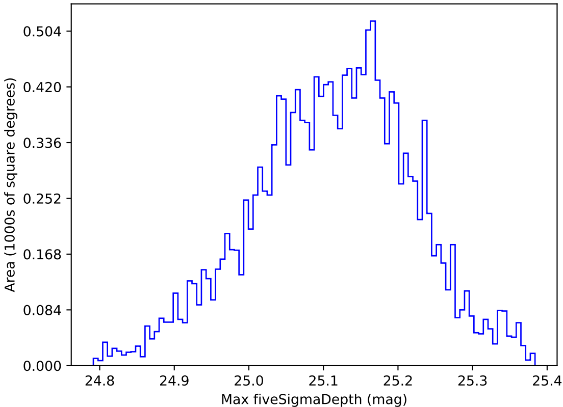
noroll_mjdp365_v3.4_10yrs WFD g band: Max fiveSigmaDepth
