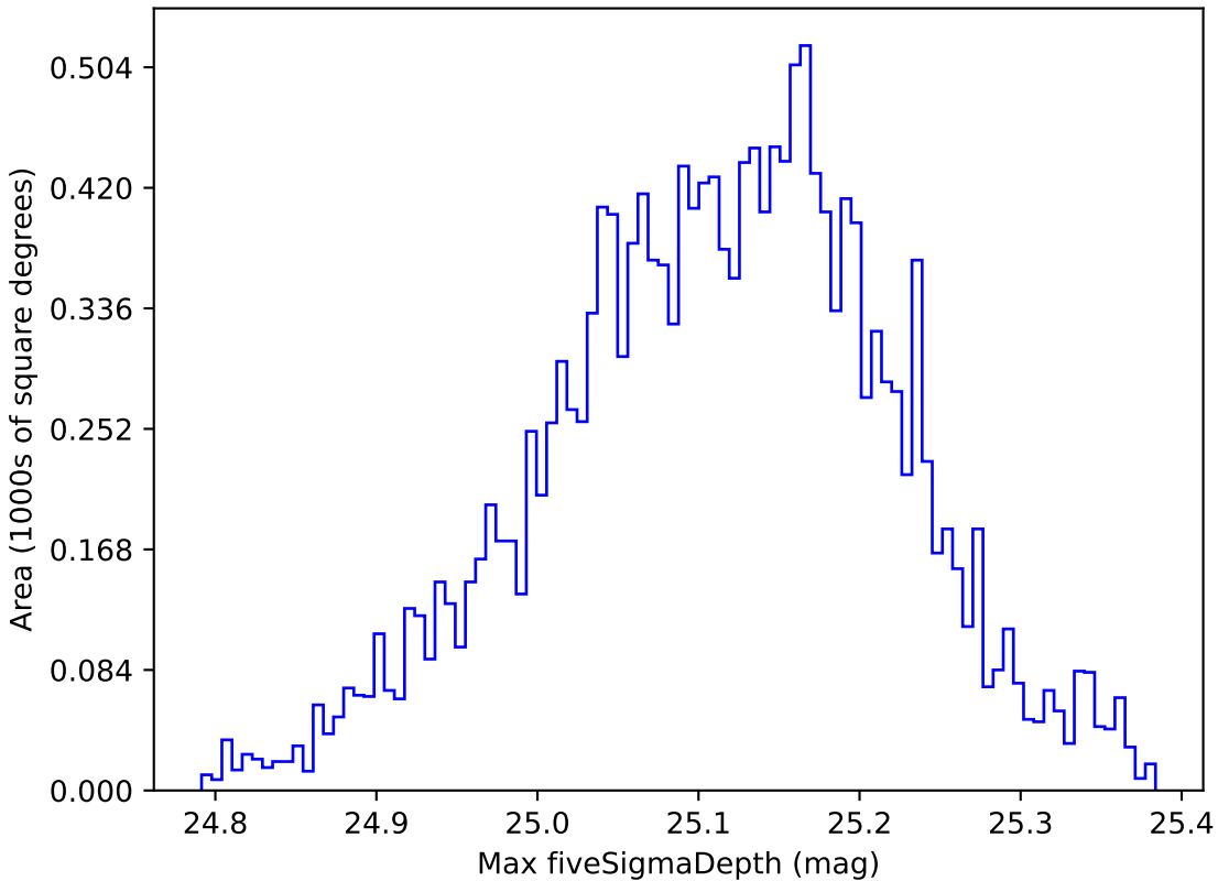
noroll_mjdp365_v3.4_10yrs WFD all bands: Max fiveSigmaDepth
