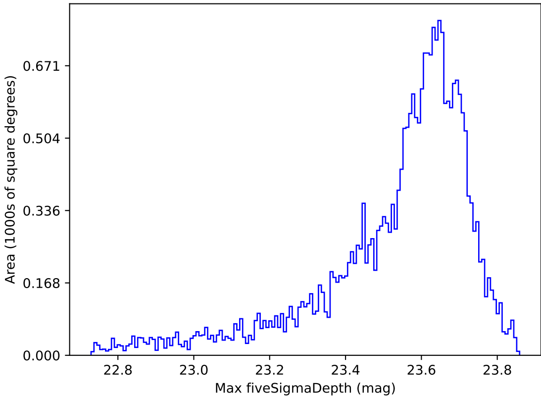
noroll_mjdp365_v3.4_10yrs All sky z band: Max fiveSigmaDepth
