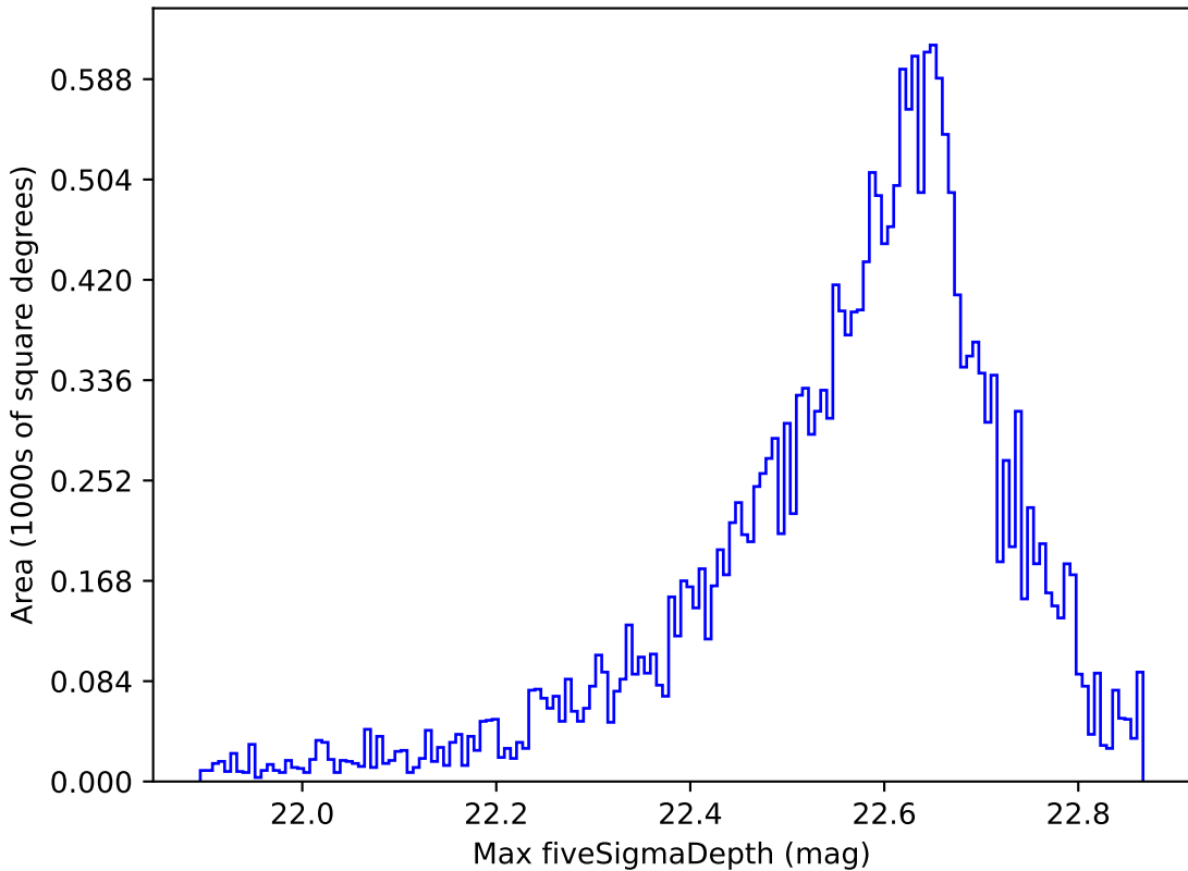
noroll_mjdp365_v3.4_10yrs All sky y band: Max fiveSigmaDepth
