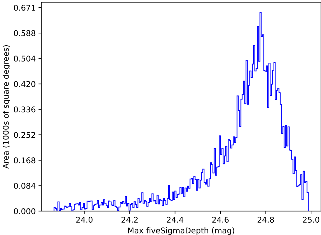
noroll_mjdp365_v3.4_10yrs All sky r band: Max fiveSigmaDepth
