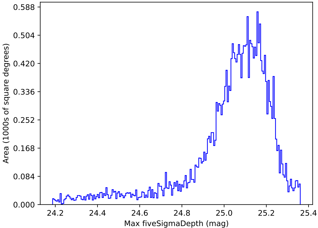
noroll_mjdp365_v3.4_10yrs All sky g band: Max fiveSigmaDepth
