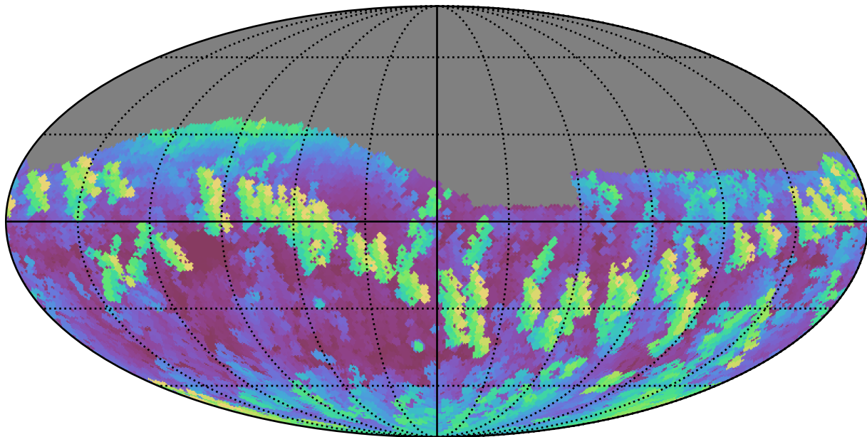
noroll_mjdp365_v3.4_10yrs Yr 1 z band: Max airmass
