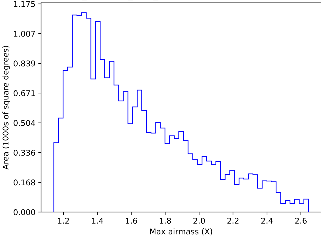
noroll_mjdp365_v3.4_10yrs Yr 1 y band: Max airmass
