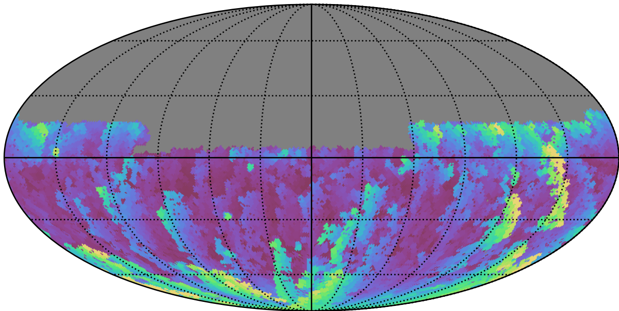
noroll_mjdp365_v3.4_10yrs Yr 1 u band: Max airmass
