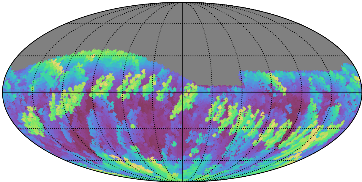
noroll_mjdp365_v3.4_10yrs Yr 1 r band: Max airmass
