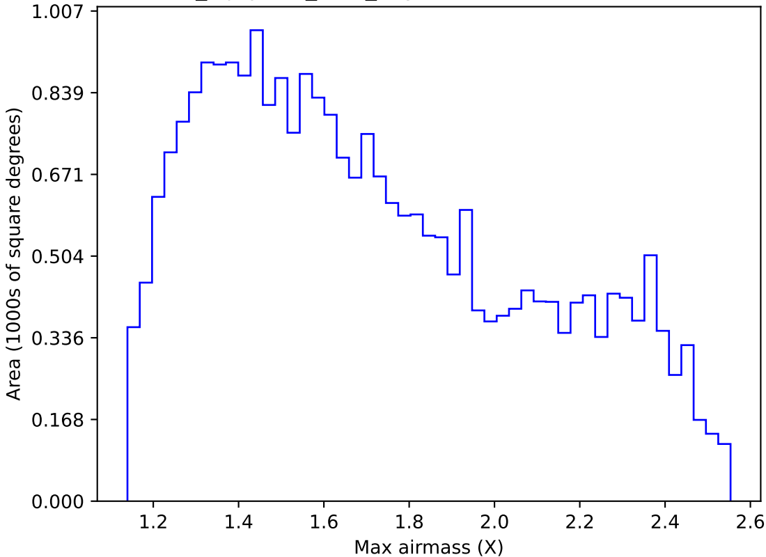
noroll_mjdp365_v3.4_10yrs Yr 1 r band: Max airmass
