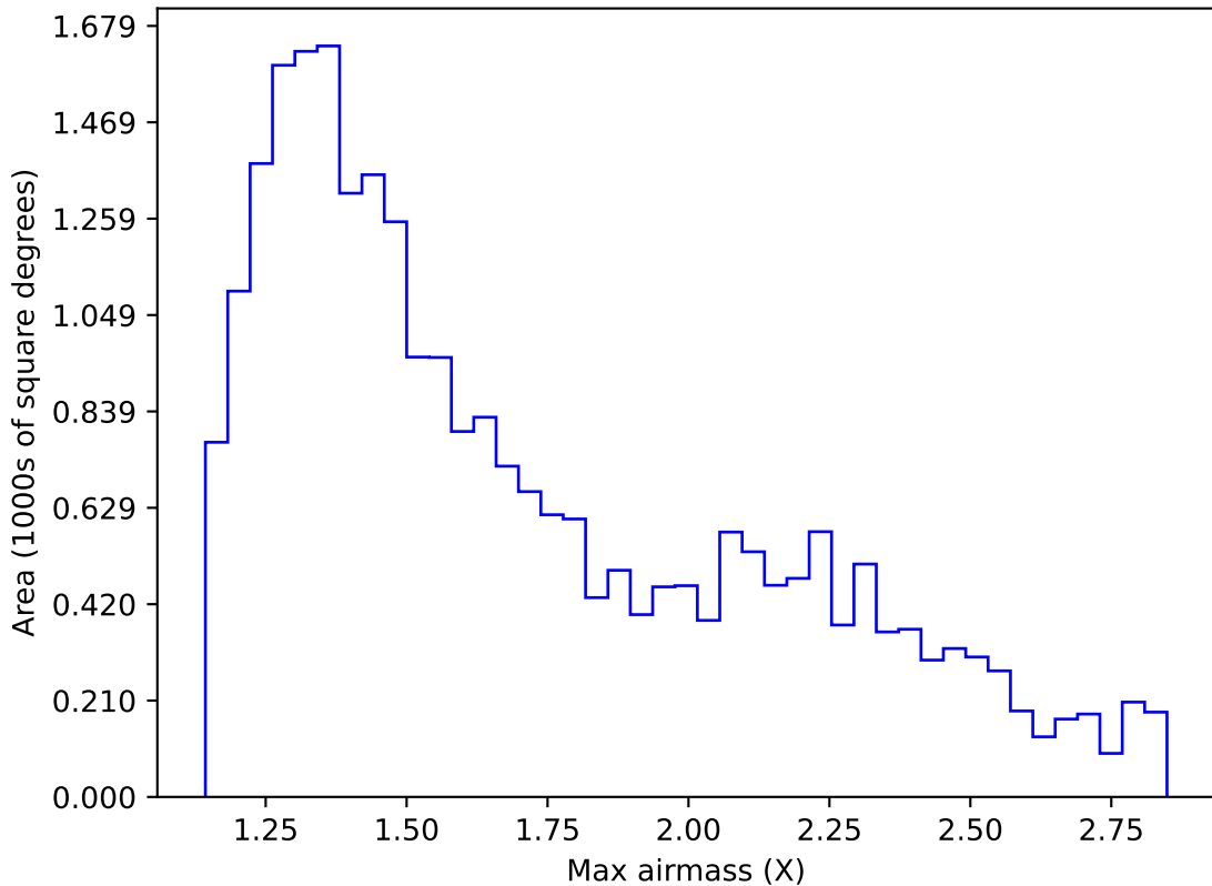
noroll_mjdp365_v3.4_10yrs Yr 1 i band: Max airmass
