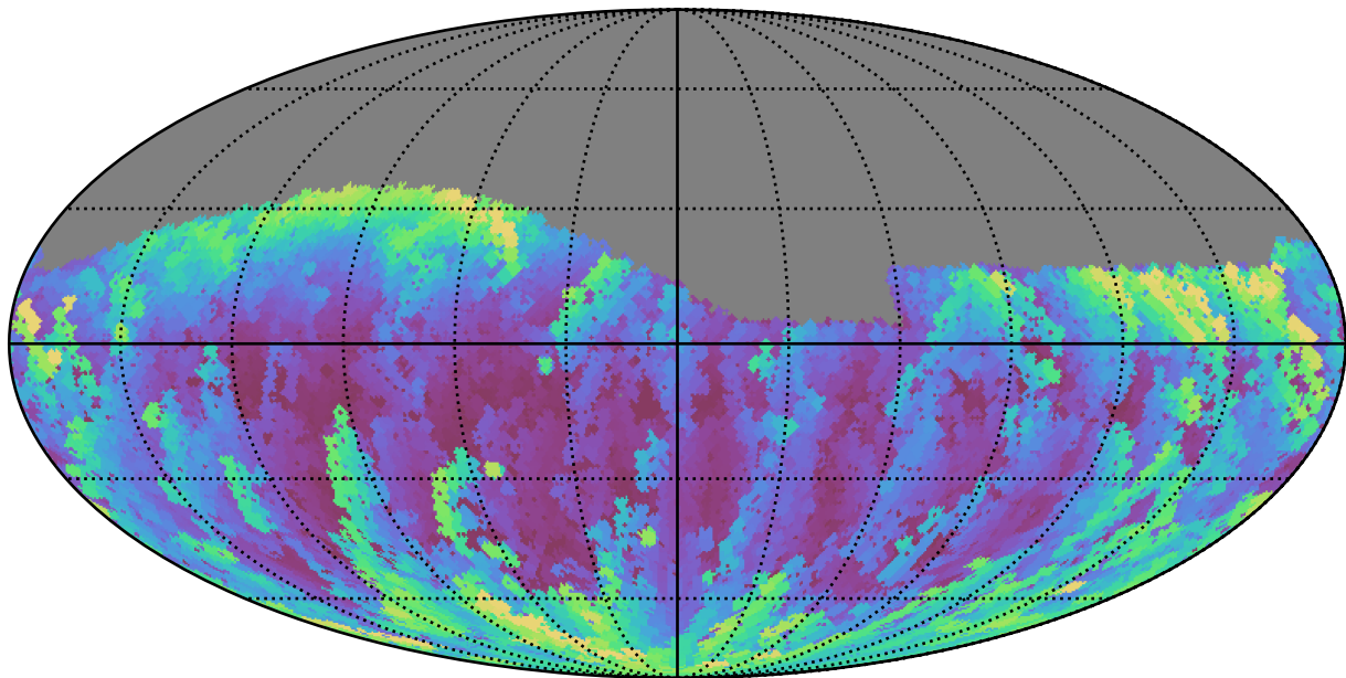
noroll_mjdp365_v3.4_10yrs Yr 1 g band: Max airmass
