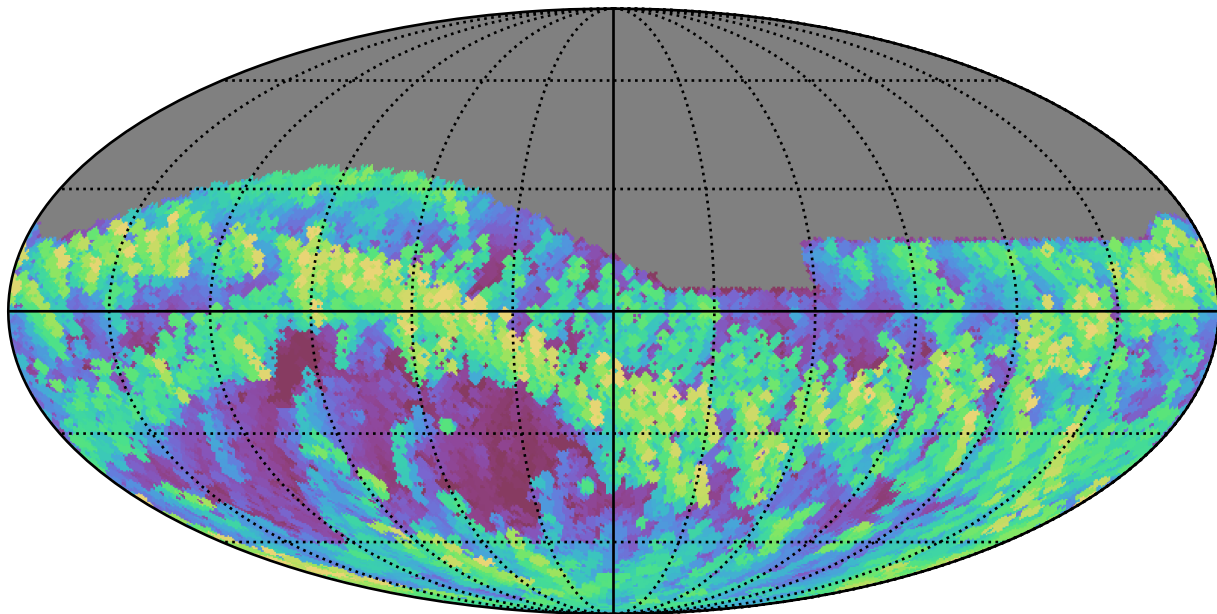
noroll_mjdp365_v3.4_10yrs Yr 1 all bands: Max airmass
