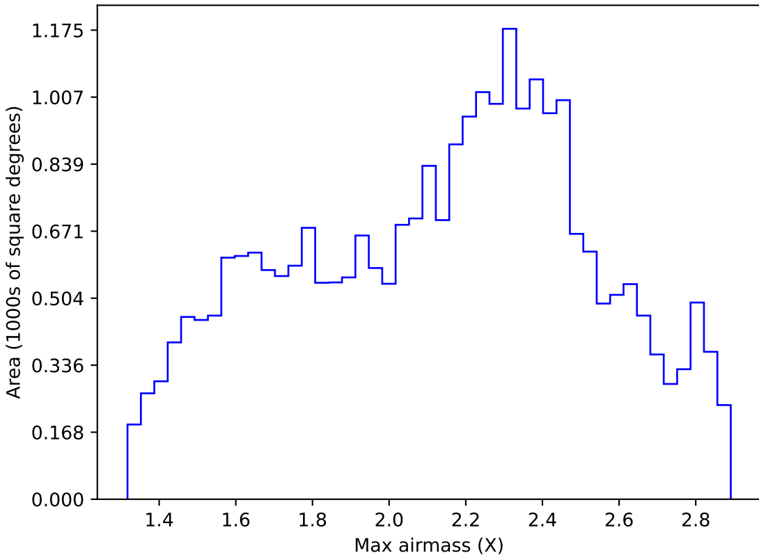
noroll_mjdp365_v3.4_10yrs Yr 1 all bands: Max airmass
