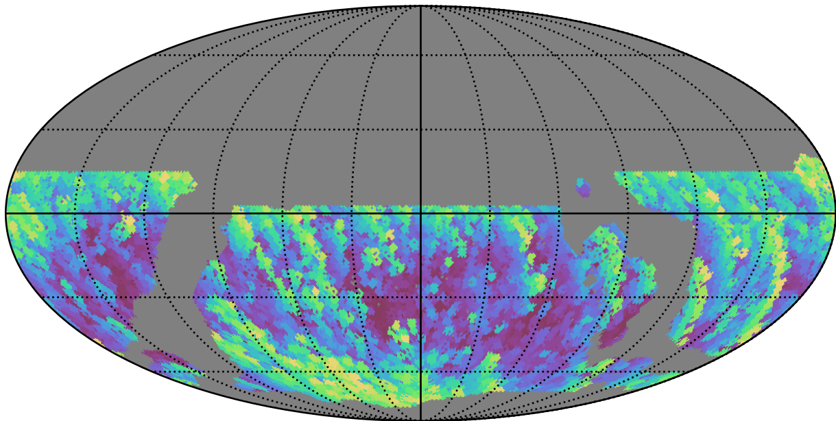
noroll_mjdp365_v3.4_10yrs WFD y band: Max airmass
