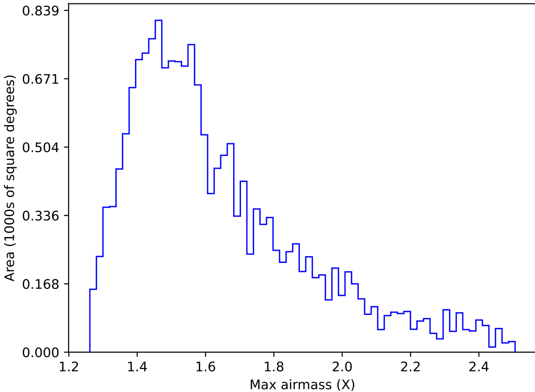
noroll_mjdp365_v3.4_10yrs WFD u band: Max airmass
