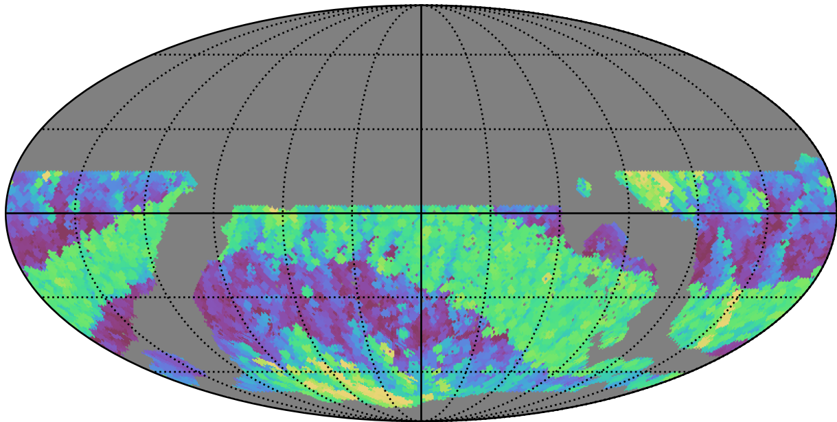
noroll_mjdp365_v3.4_10yrs WFD r band: Max airmass
