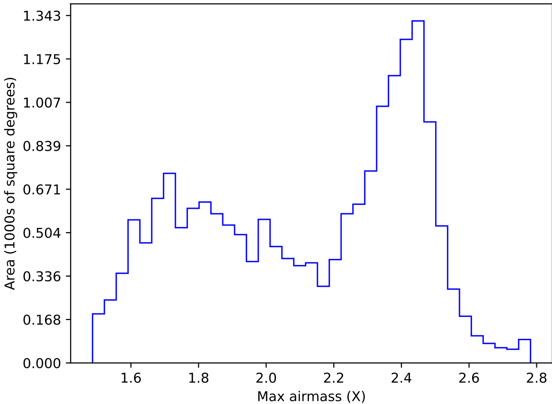
noroll_mjdp365_v3.4_10yrs WFD r band: Max airmass
