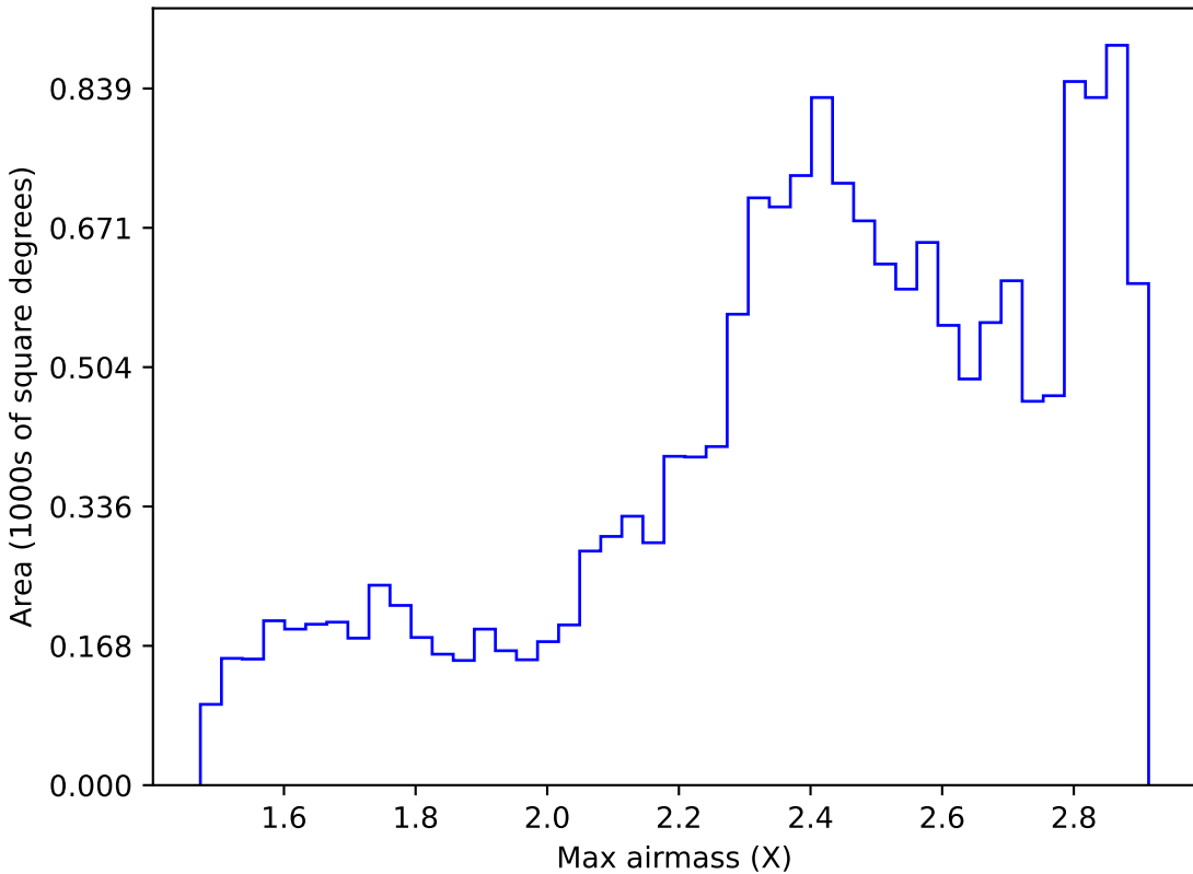
noroll_mjdp365_v3.4_10yrs WFD i band: Max airmass
