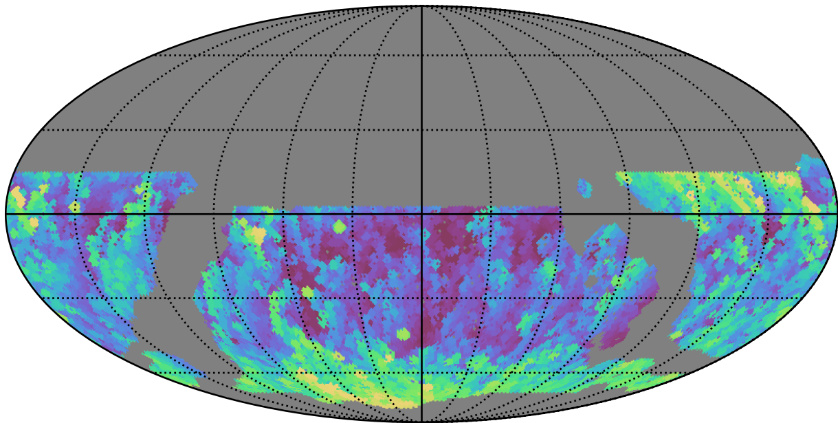
noroll_mjdp365_v3.4_10yrs WFD g band: Max airmass
