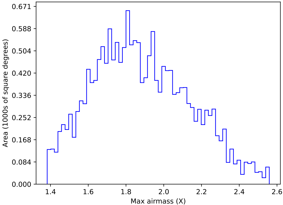
noroll_mjdp365_v3.4_10yrs WFD g band: Max airmass
