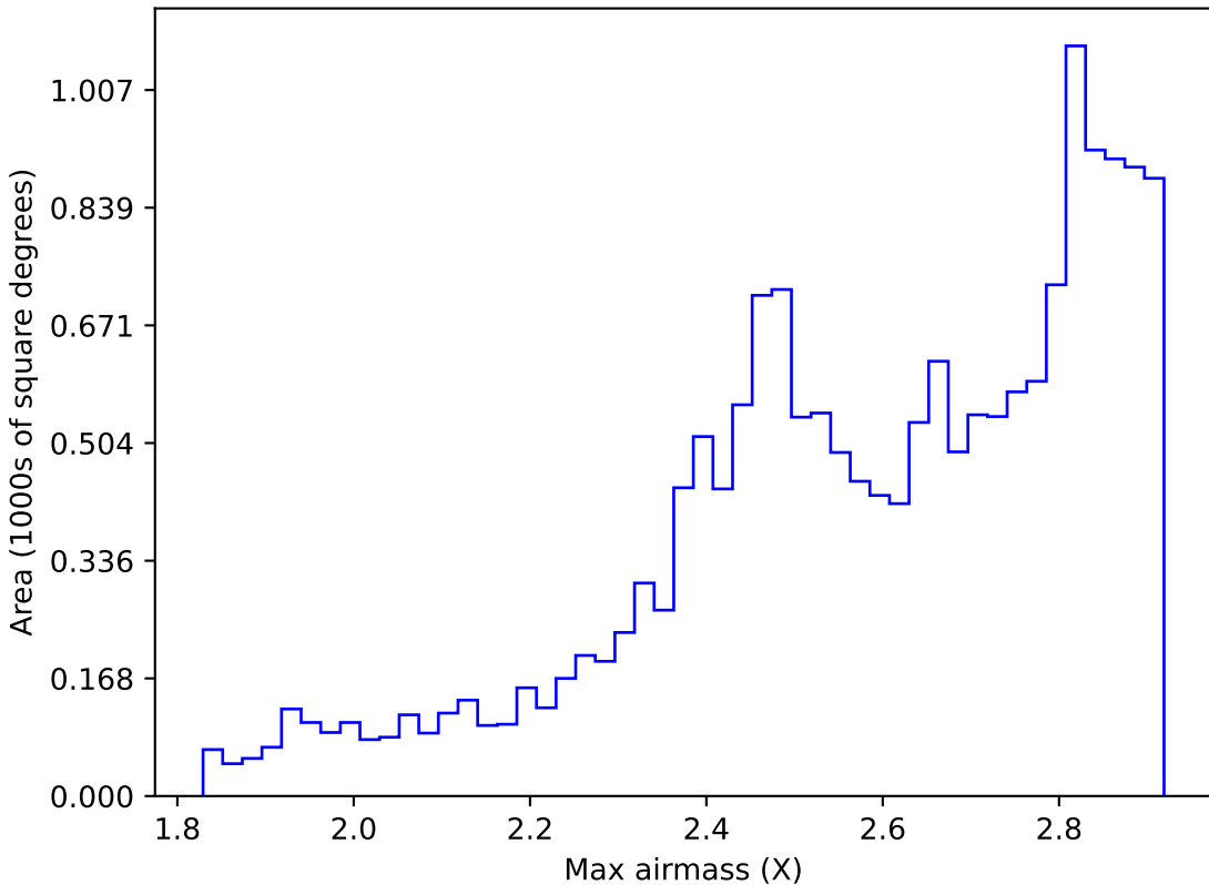
noroll_mjdp365_v3.4_10yrs WFD all bands: Max airmass
