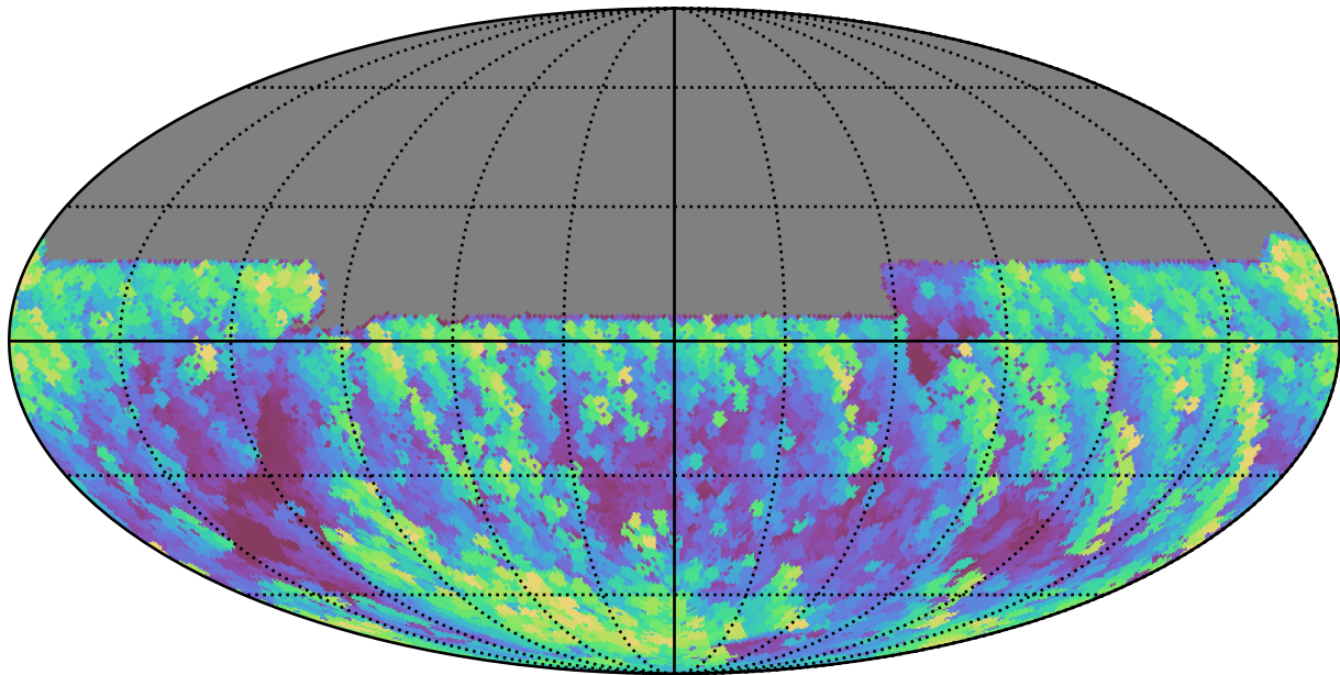
noroll_mjdp365_v3.4_10yrs All sky y band: Max airmass
