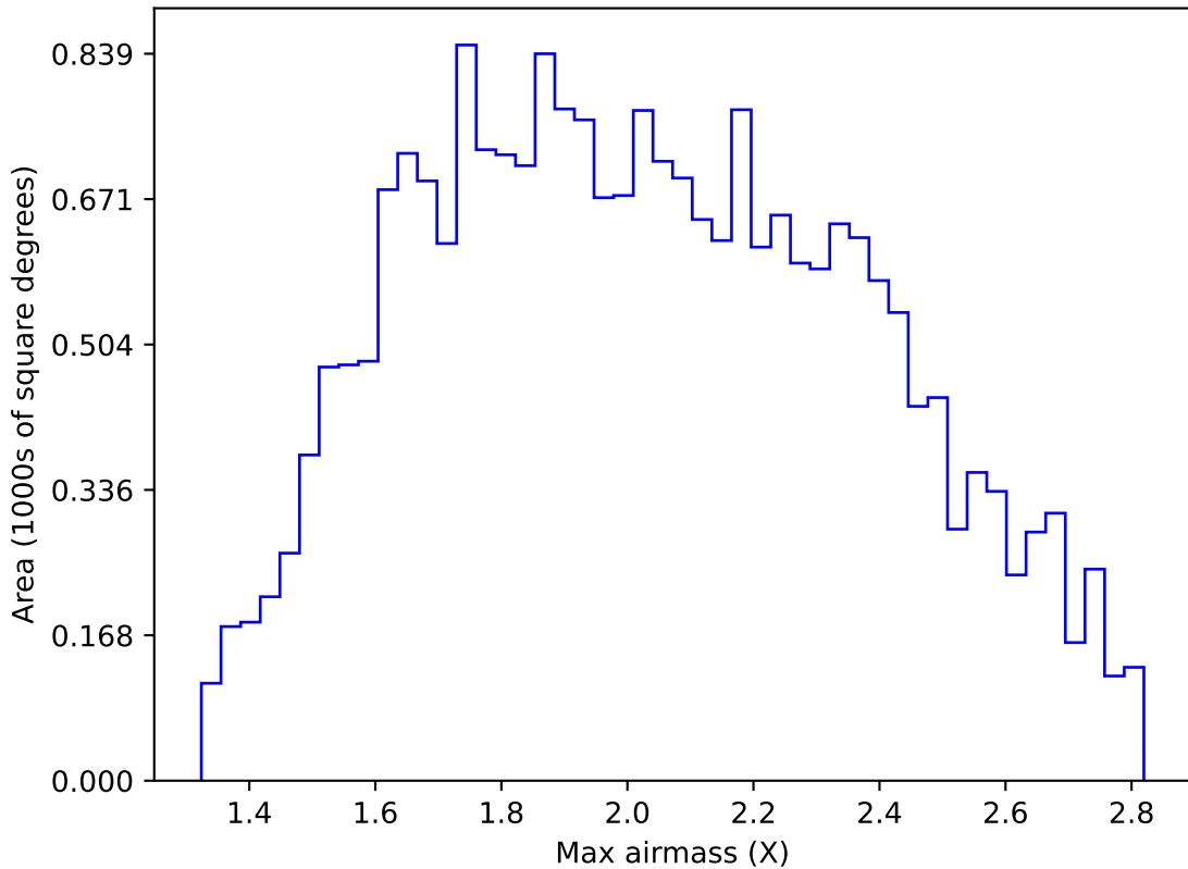
noroll_mjdp365_v3.4_10yrs All sky y band: Max airmass
