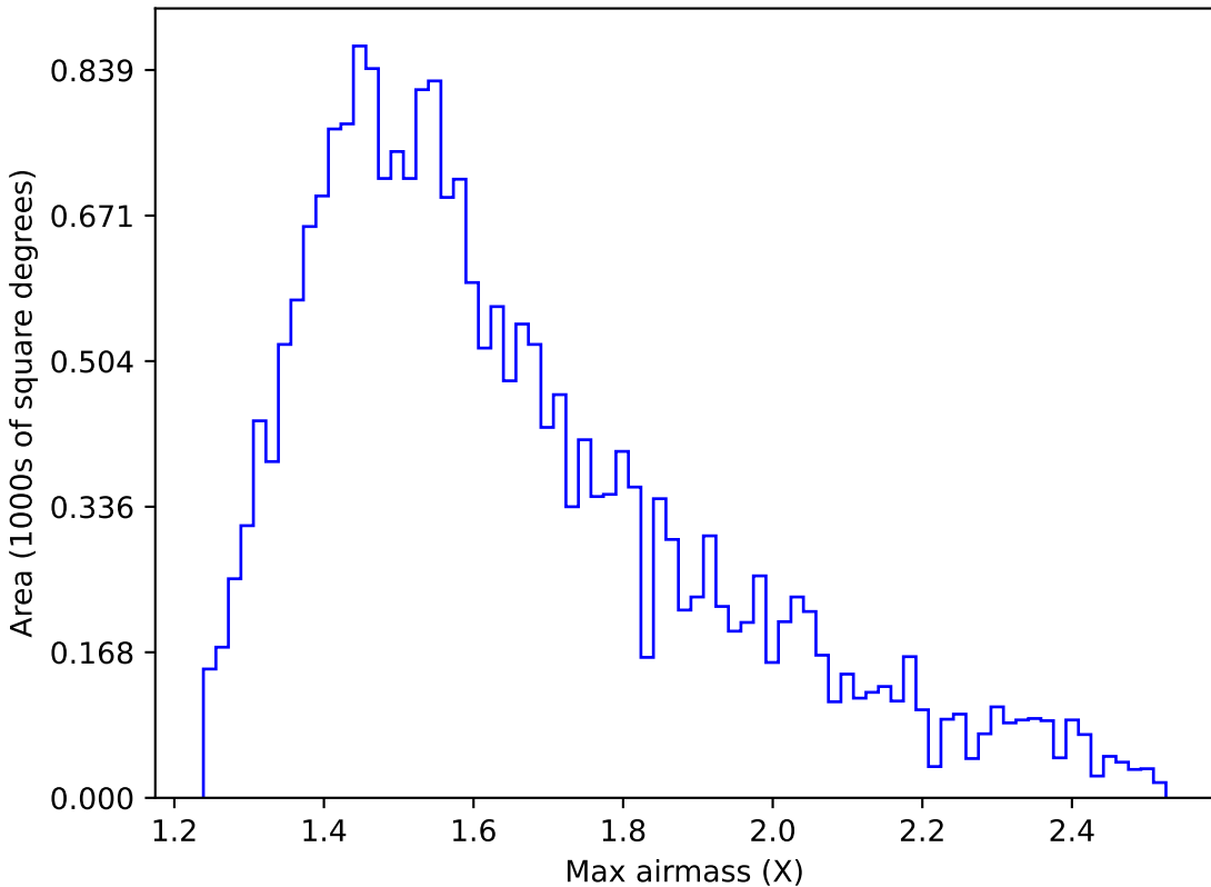
noroll_mjdp365_v3.4_10yrs All sky u band: Max airmass
