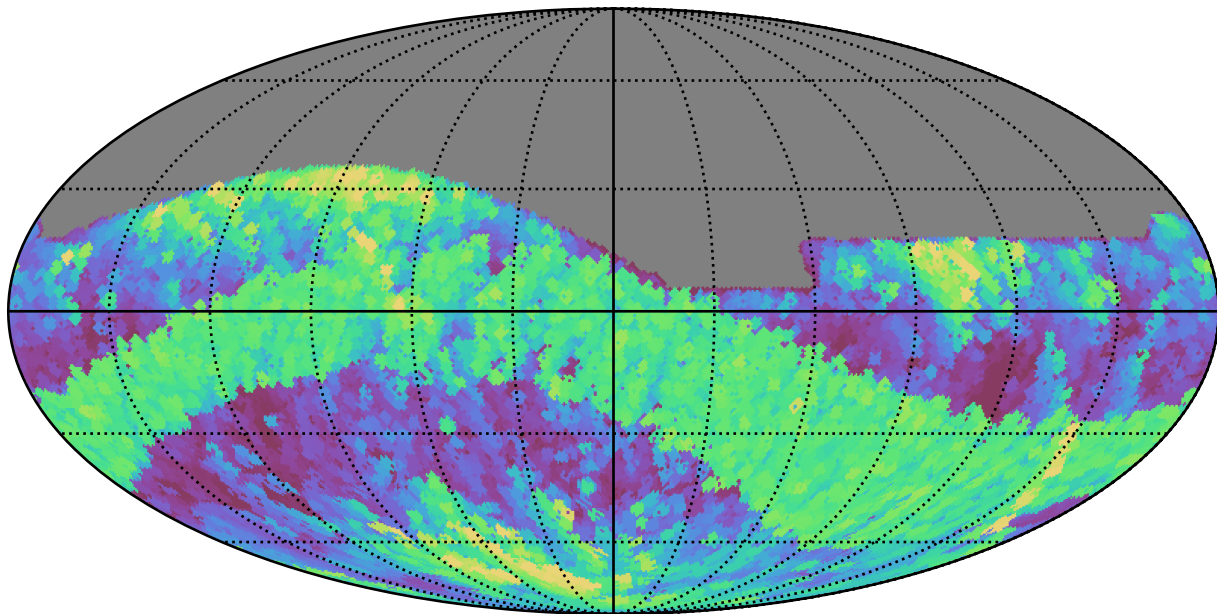
noroll_mjdp365_v3.4_10yrs All sky r band: Max airmass
