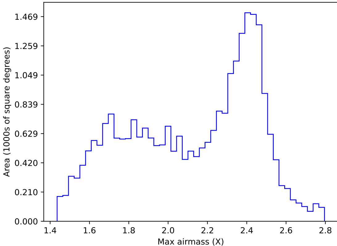
noroll_mjdp365_v3.4_10yrs All sky r band: Max airmass
