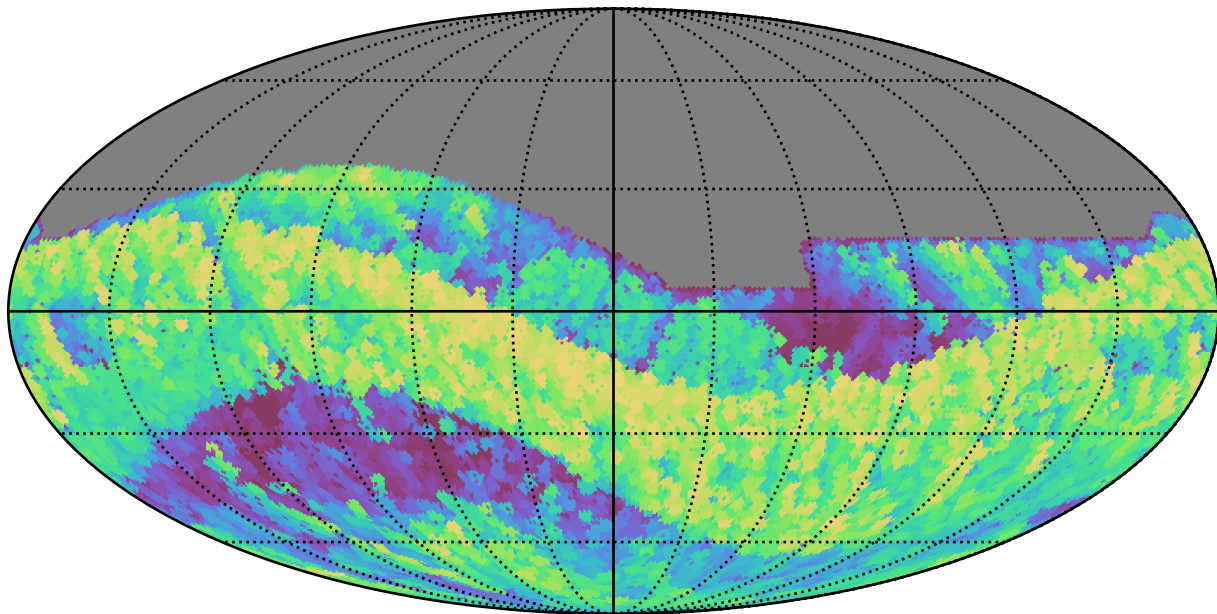
noroll_mjdp365_v3.4_10yrs All sky i band: Max airmass
