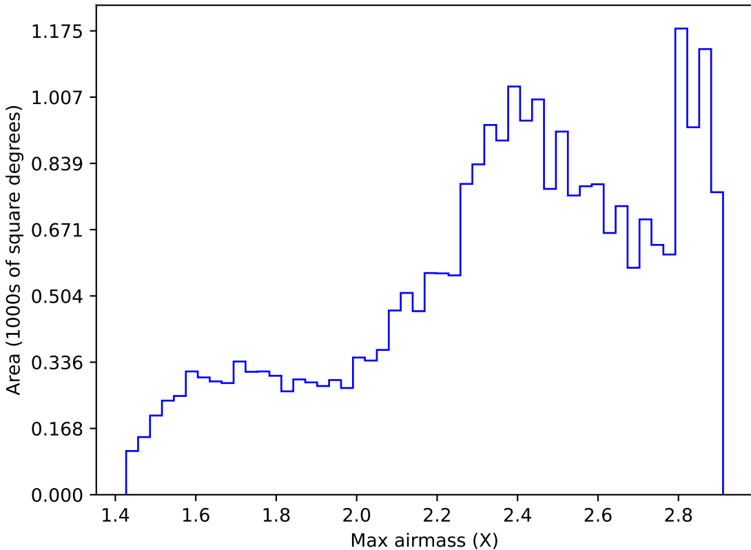
noroll_mjdp365_v3.4_10yrs All sky i band: Max airmass
