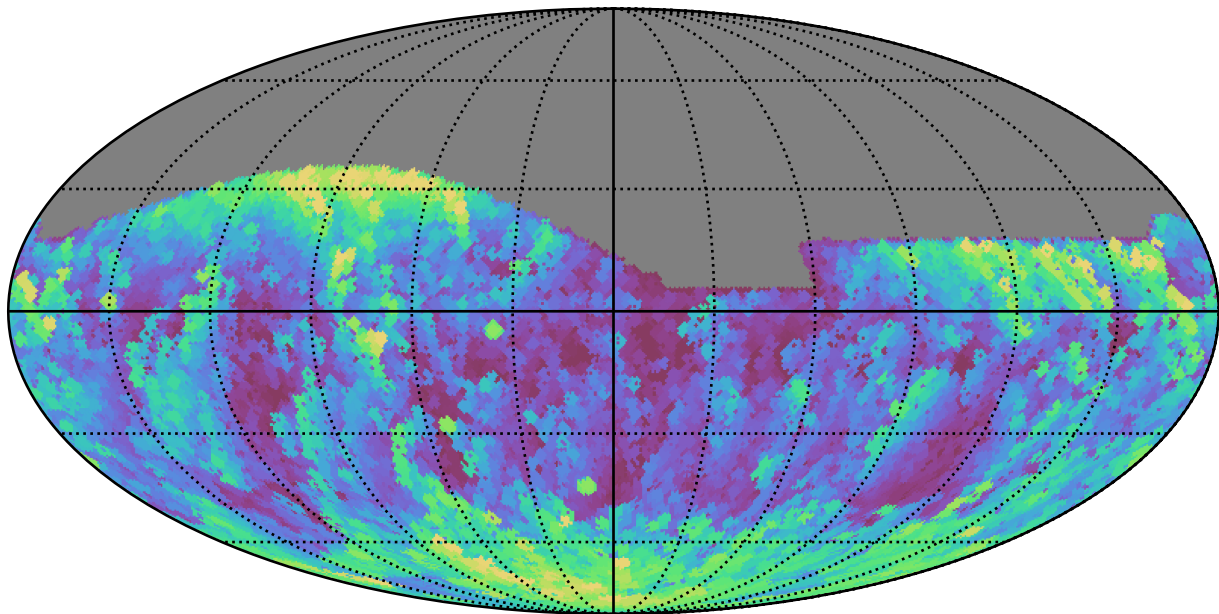
noroll_mjdp365_v3.4_10yrs All sky g band: Max airmass
