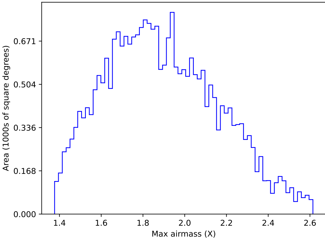
noroll_mjdp365_v3.4_10yrs All sky g band: Max airmass
