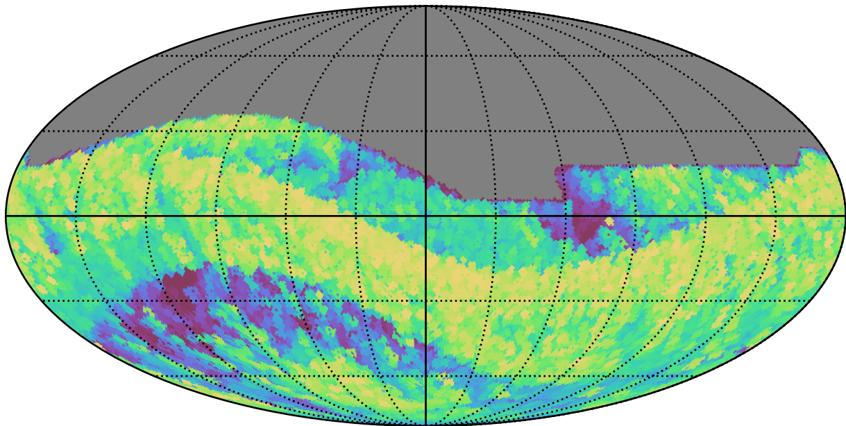
noroll_mjdp365_v3.4_10yrs All sky all bands: Max airmass
