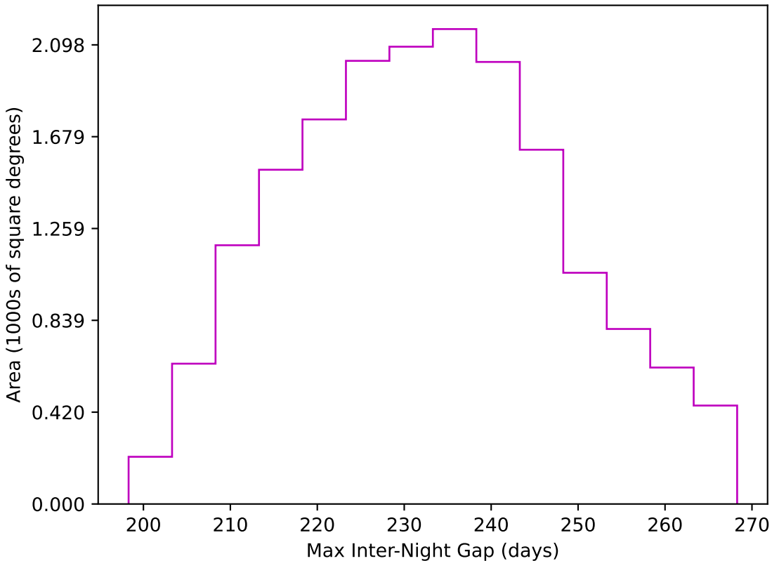
noroll_mjdp365_v3.4_10yrs WFD z band: Max Inter-Night Gap
