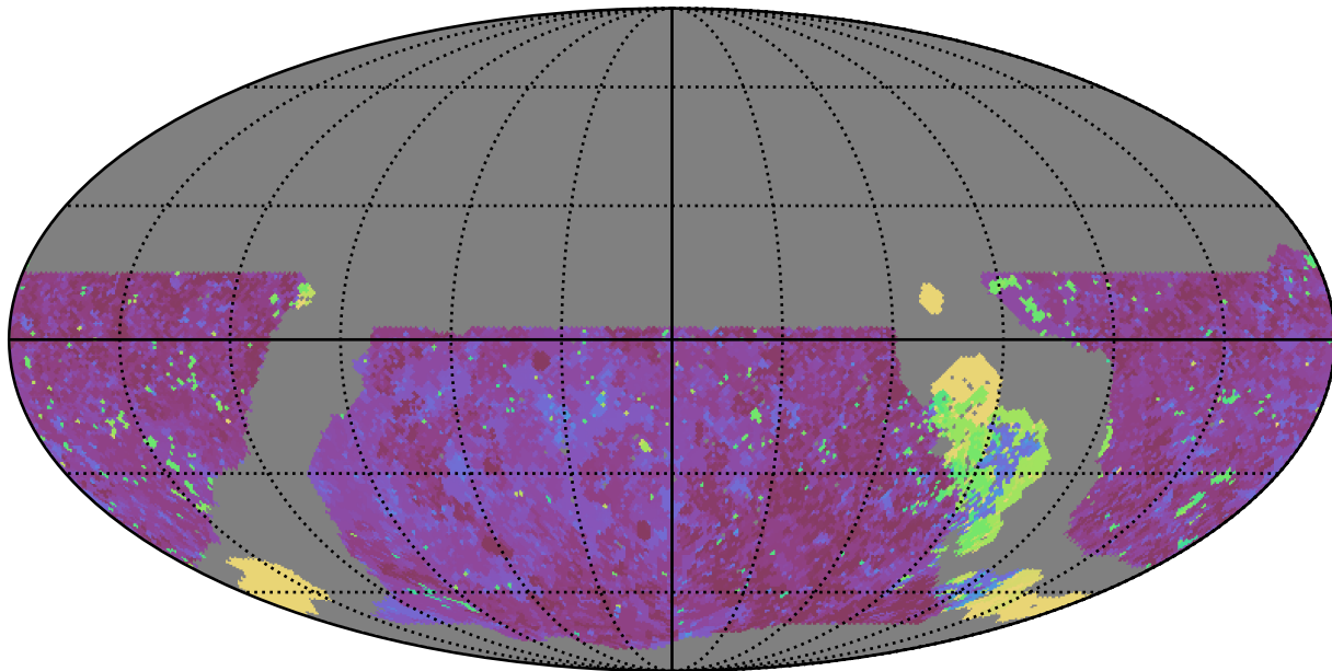
noroll_mjdp365_v3.4_10yrs WFD u band: Max Inter-Night Gap
