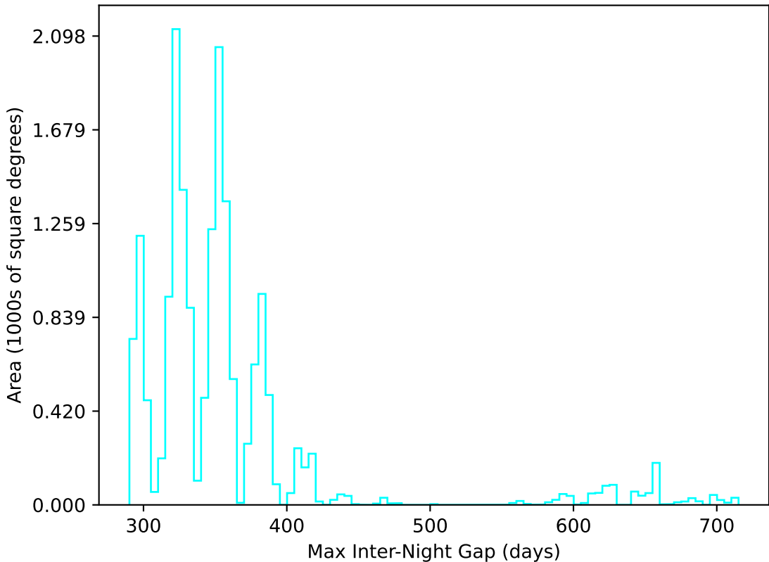
noroll_mjdp365_v3.4_10yrs WFD u band: Max Inter-Night Gap
