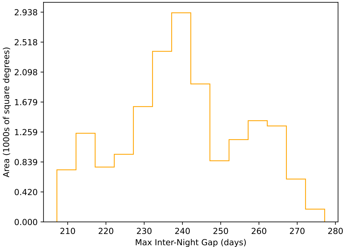
noroll_mjdp365_v3.4_10yrs WFD r band: Max Inter-Night Gap
