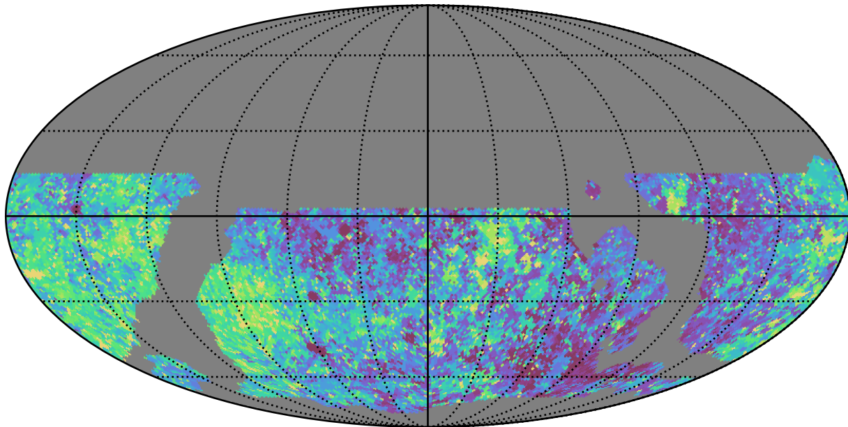
noroll_mjdp365_v3.4_10yrs WFD i band: Max Inter-Night Gap
